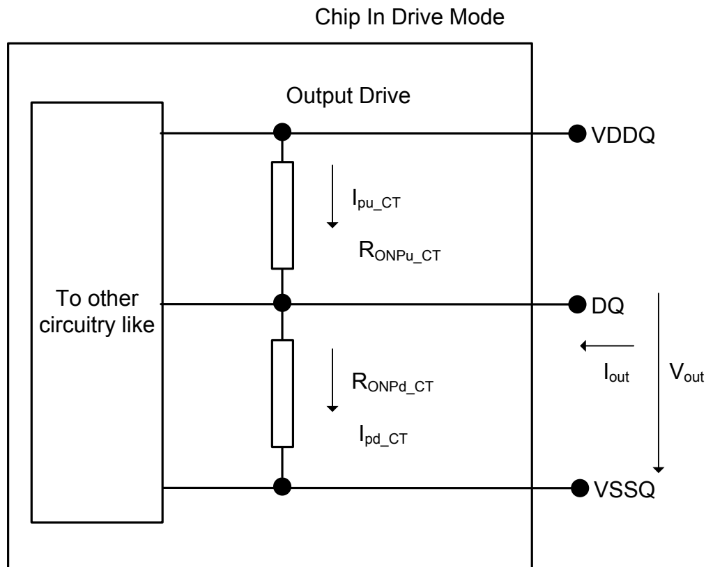
Figure 181. Output Driver Characteristic of Connectivity Test
