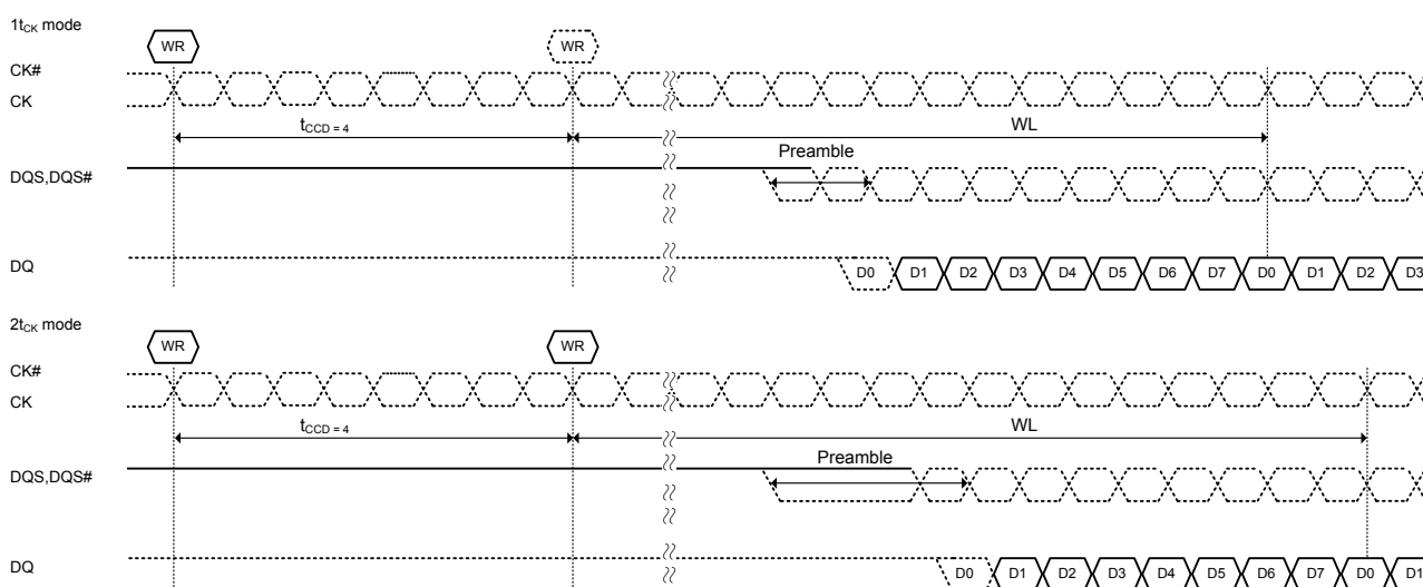
Figure 79. t_{CCD}=4 (AL=PL=0)
