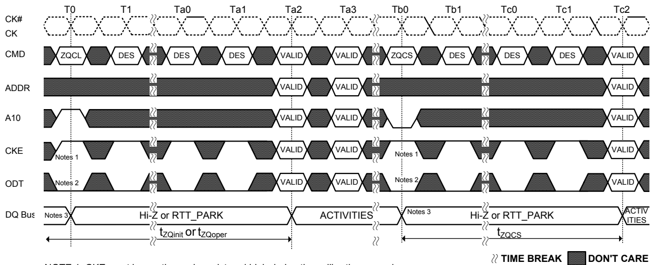
Figure 43. ZQ Calibration Timing
