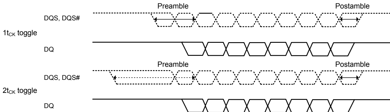
Figure 85. WRITE Postamble
