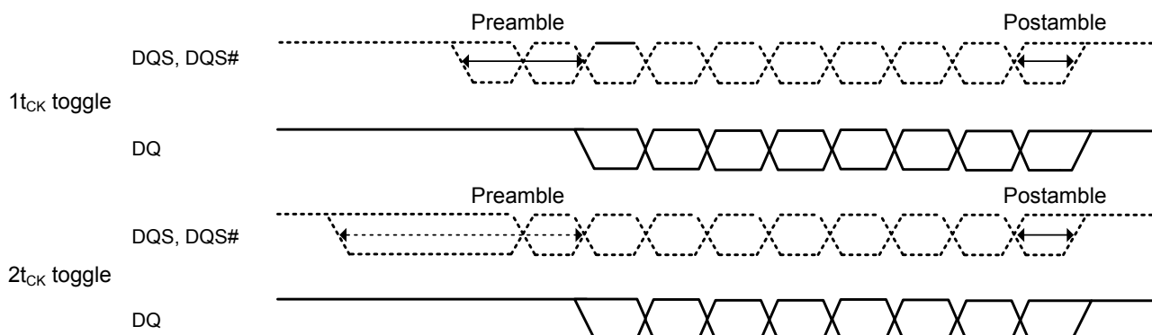
Figure 84. READ Postamble
