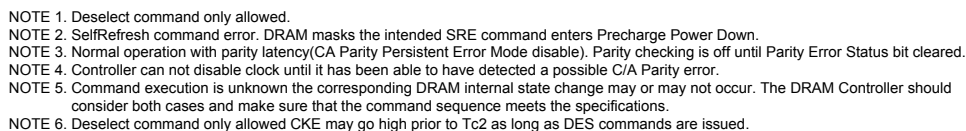
Figure 58. CA Parity Error Checking - SRE Attempt
