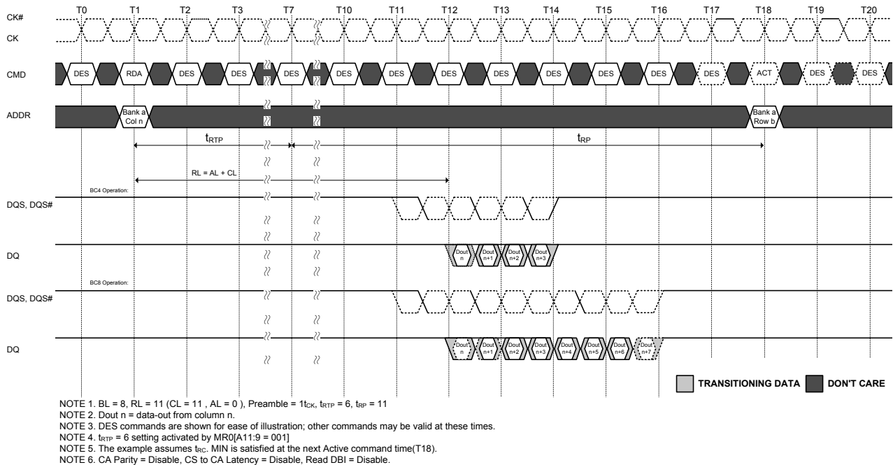
Figure 114. READ with Auto Precharge and 1t CK Preamble
